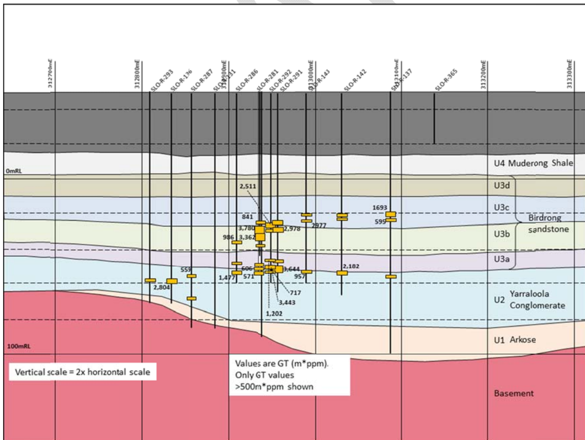
Typical cross section from the main portion of the mineralisation showing the general stratigraphy and underlying basement.
